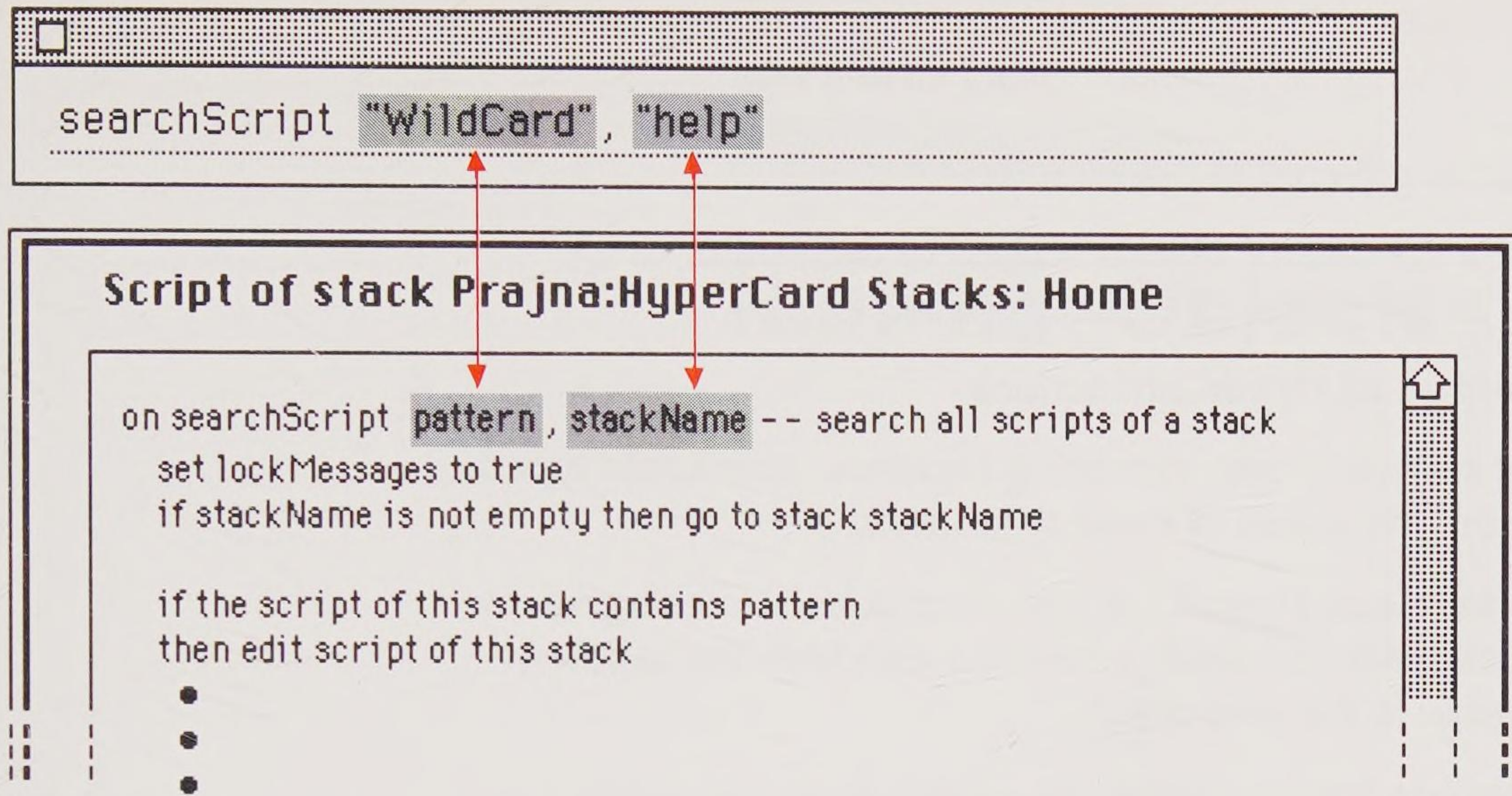
Figure 2-13 Parameter passing
