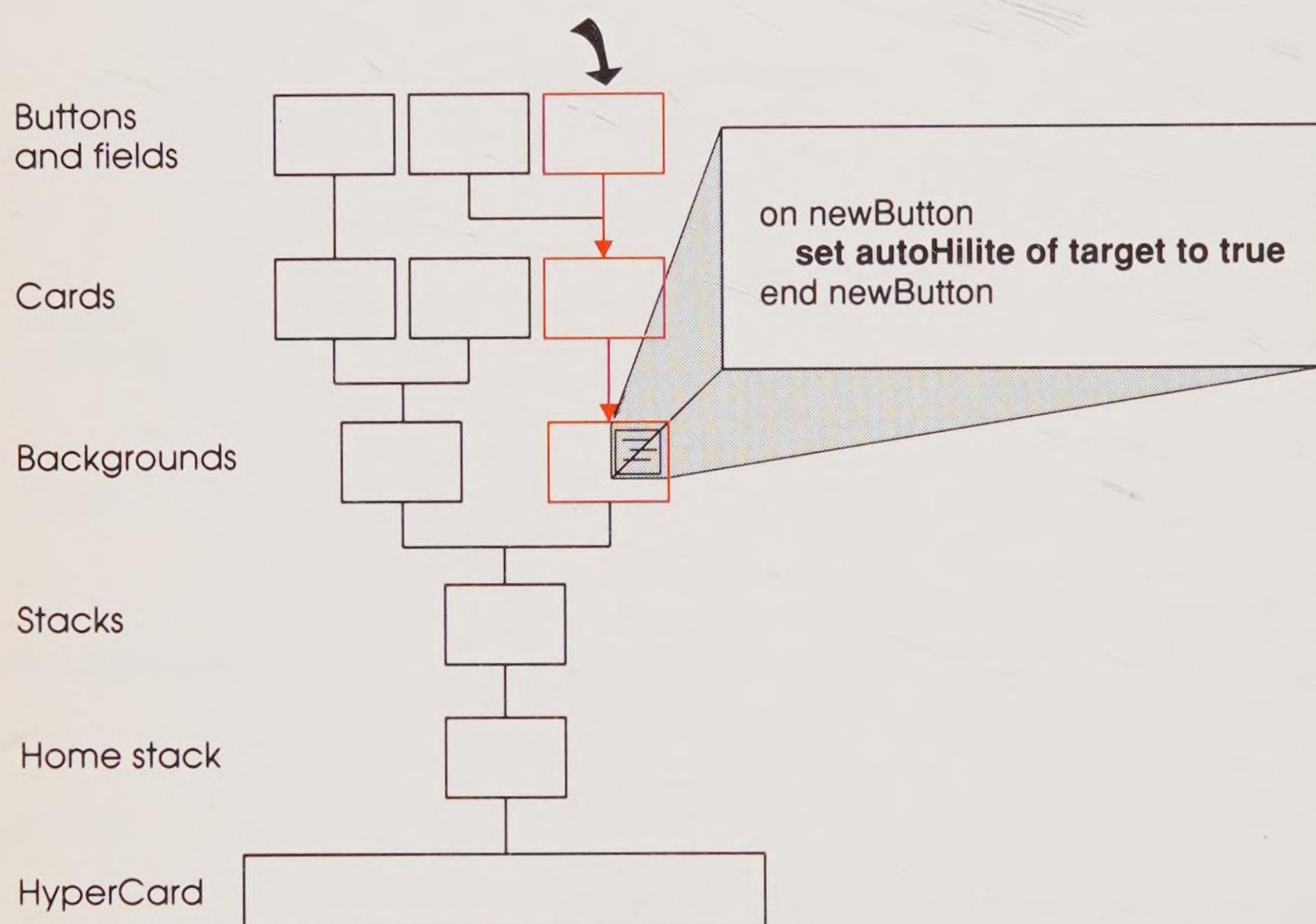
Figure 2-6 The target
