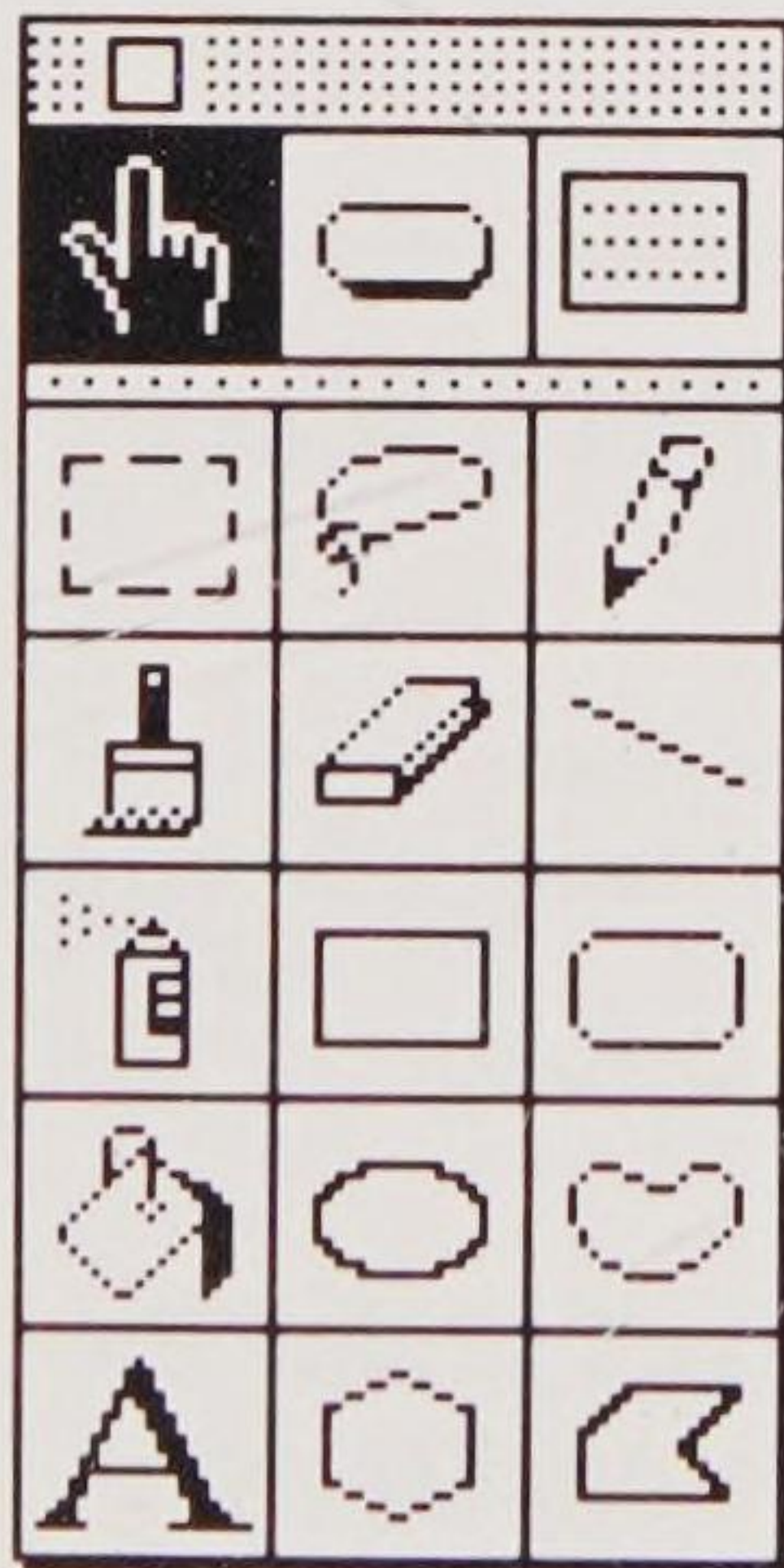
Figure 7-3 Tools palette
