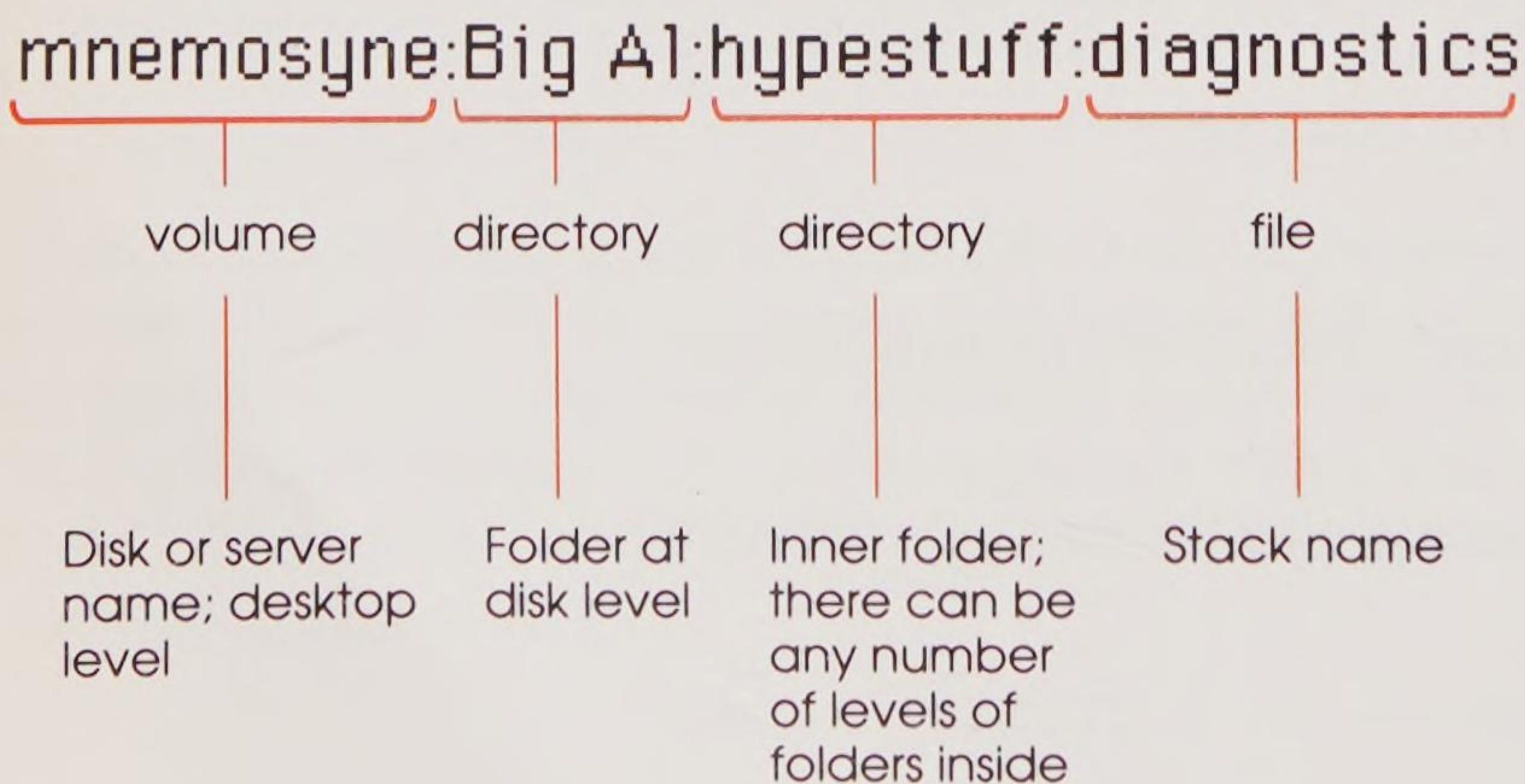
Figure 3-2 A pathname
