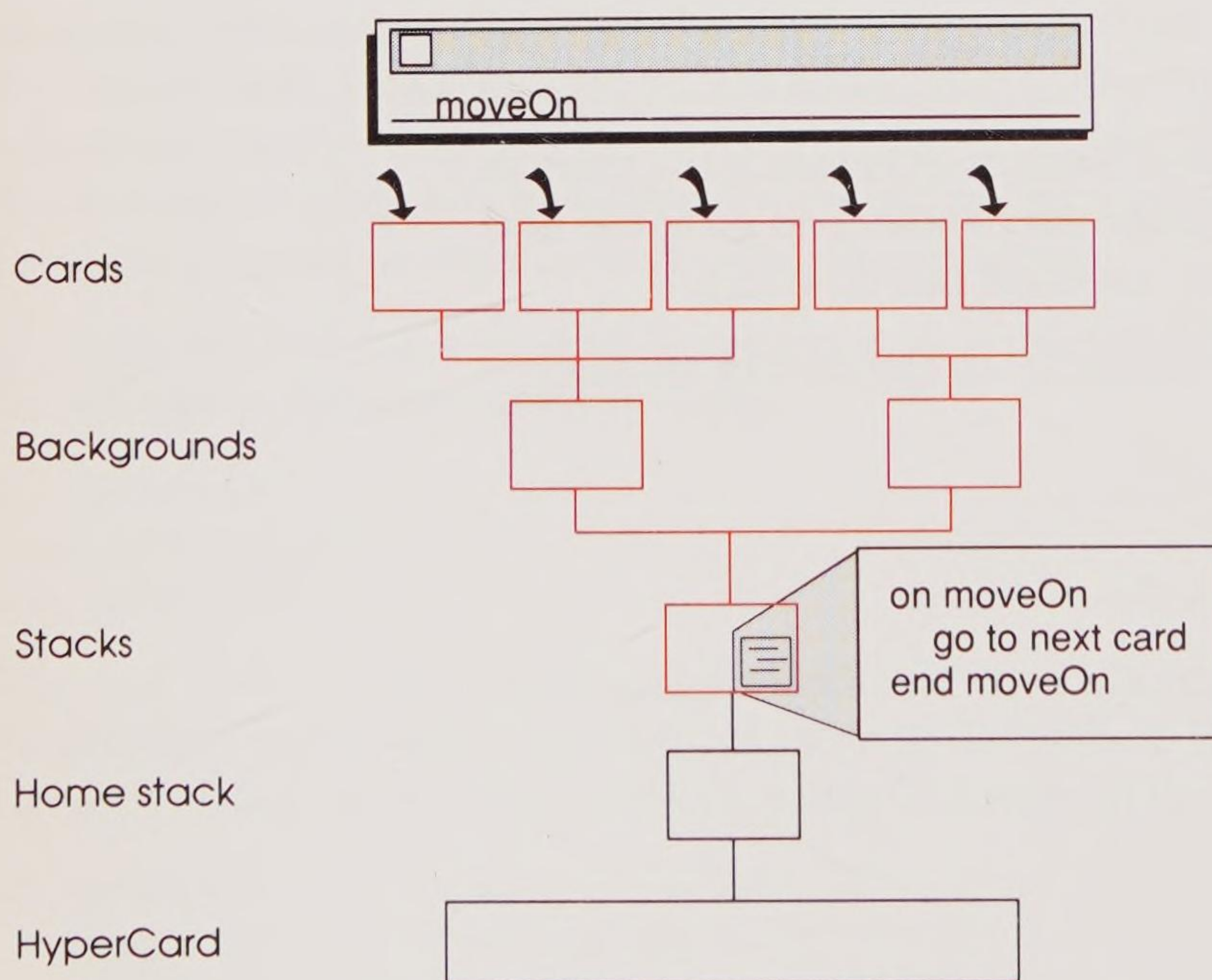
Figure 2-11 Handler in stack script
