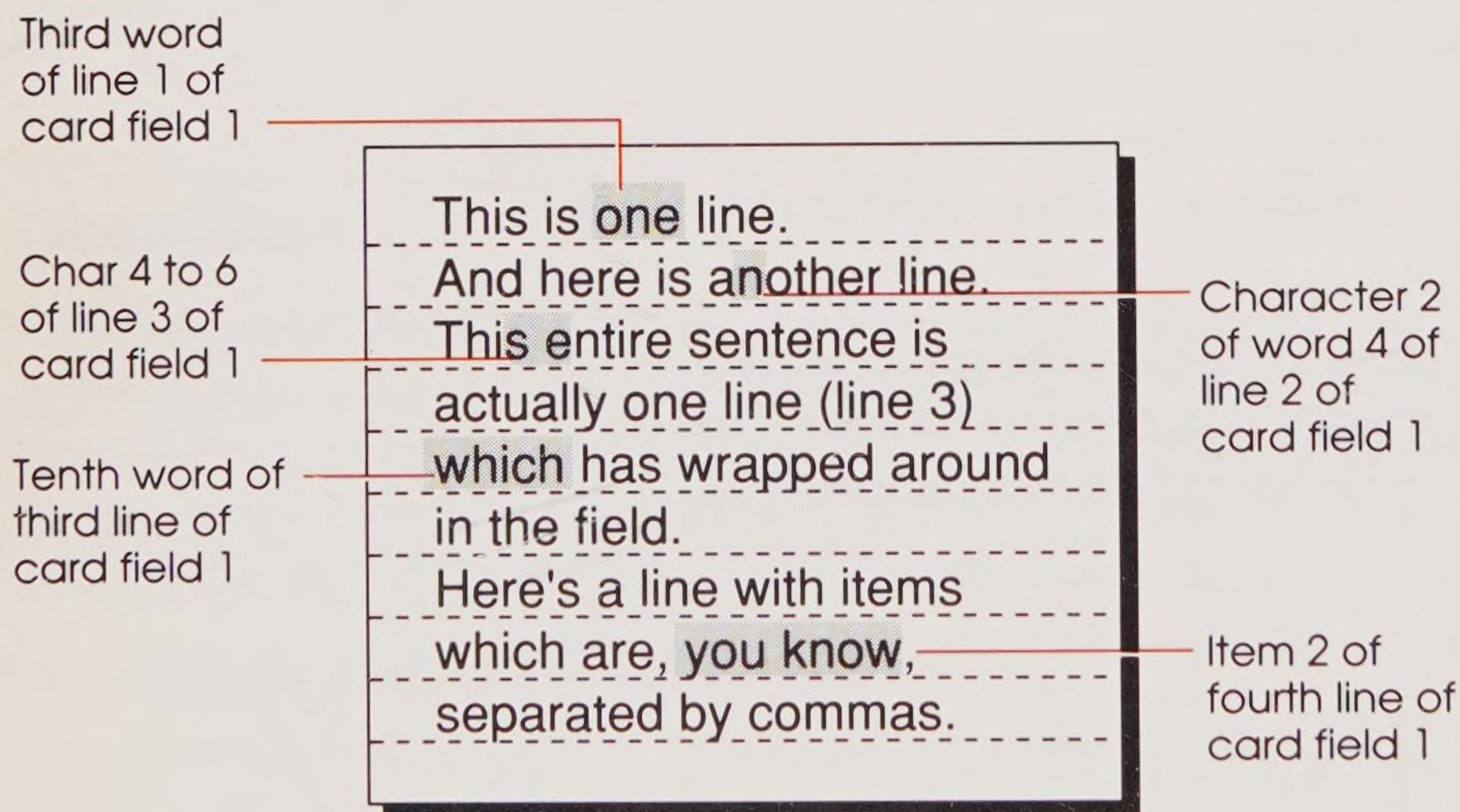
Figure 4-4 Chunk expressions
