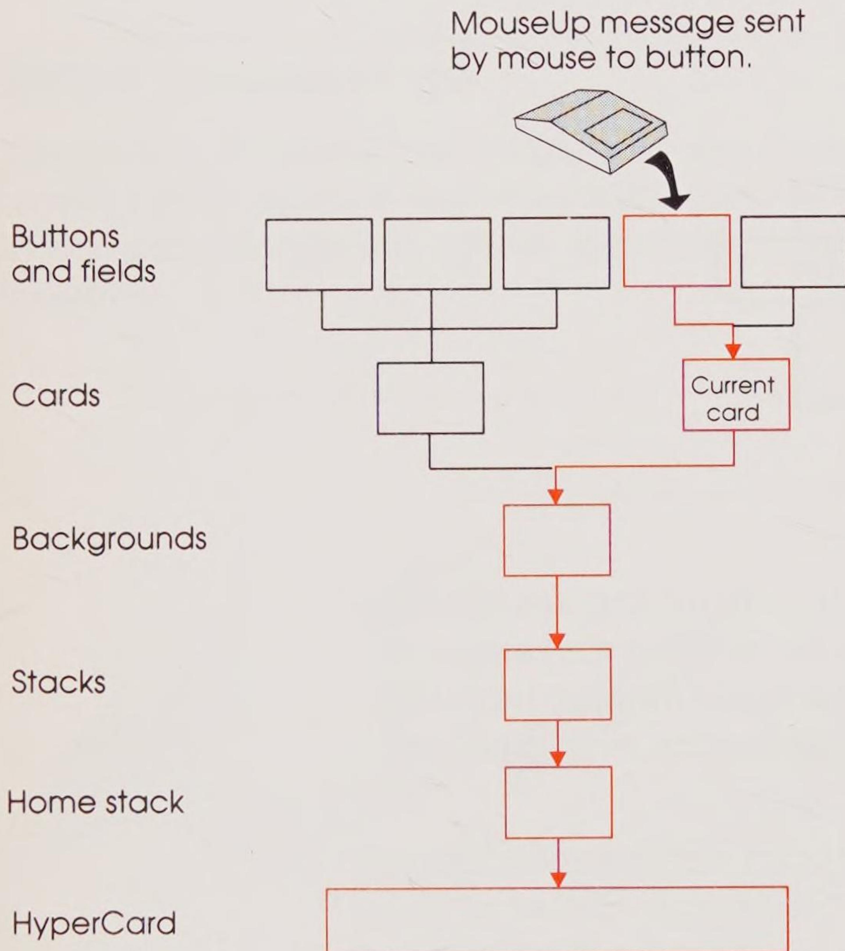
Figure 2-4 Message traversing current hierarchy
