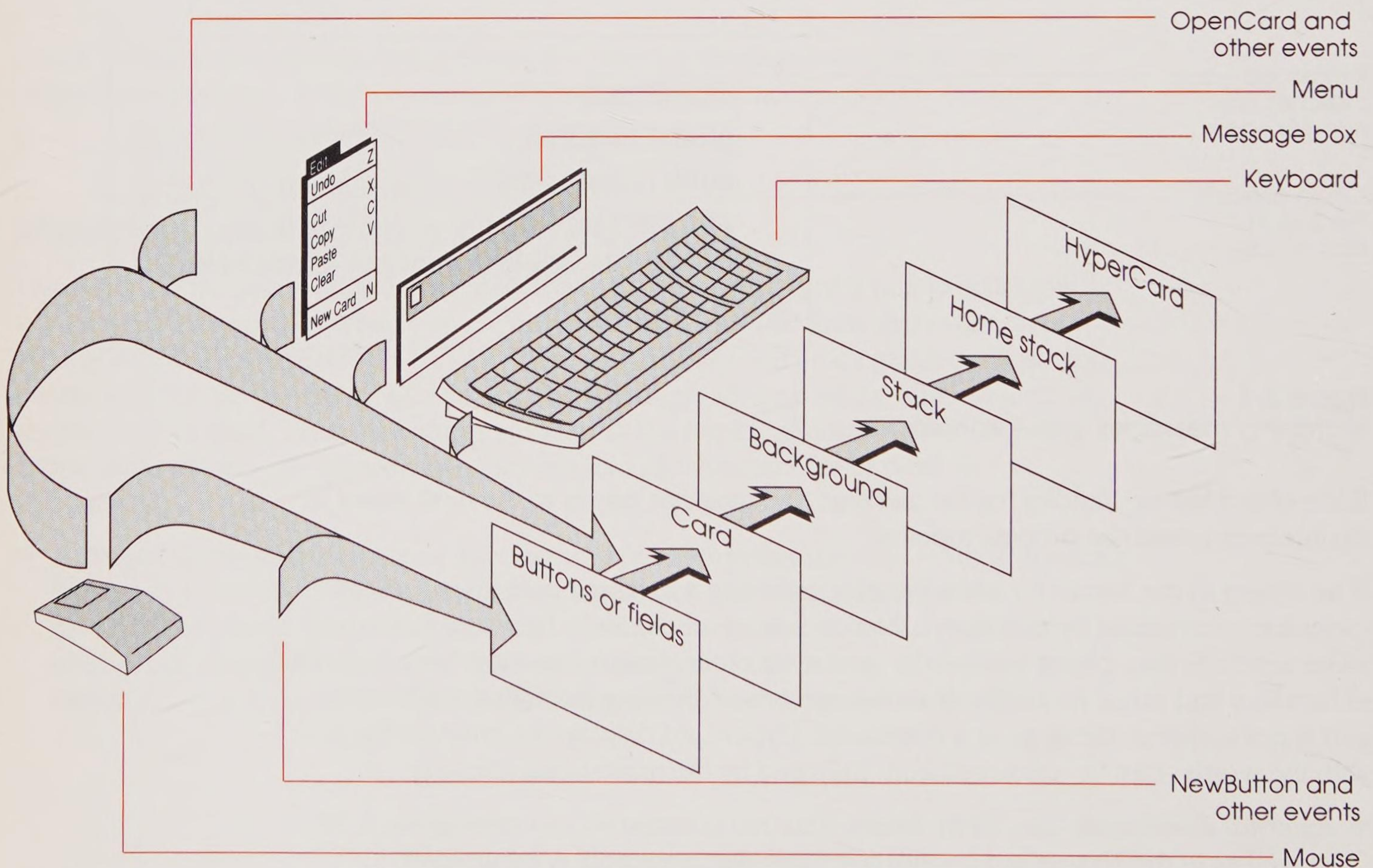
Figure 2-2 Object hierarchy
