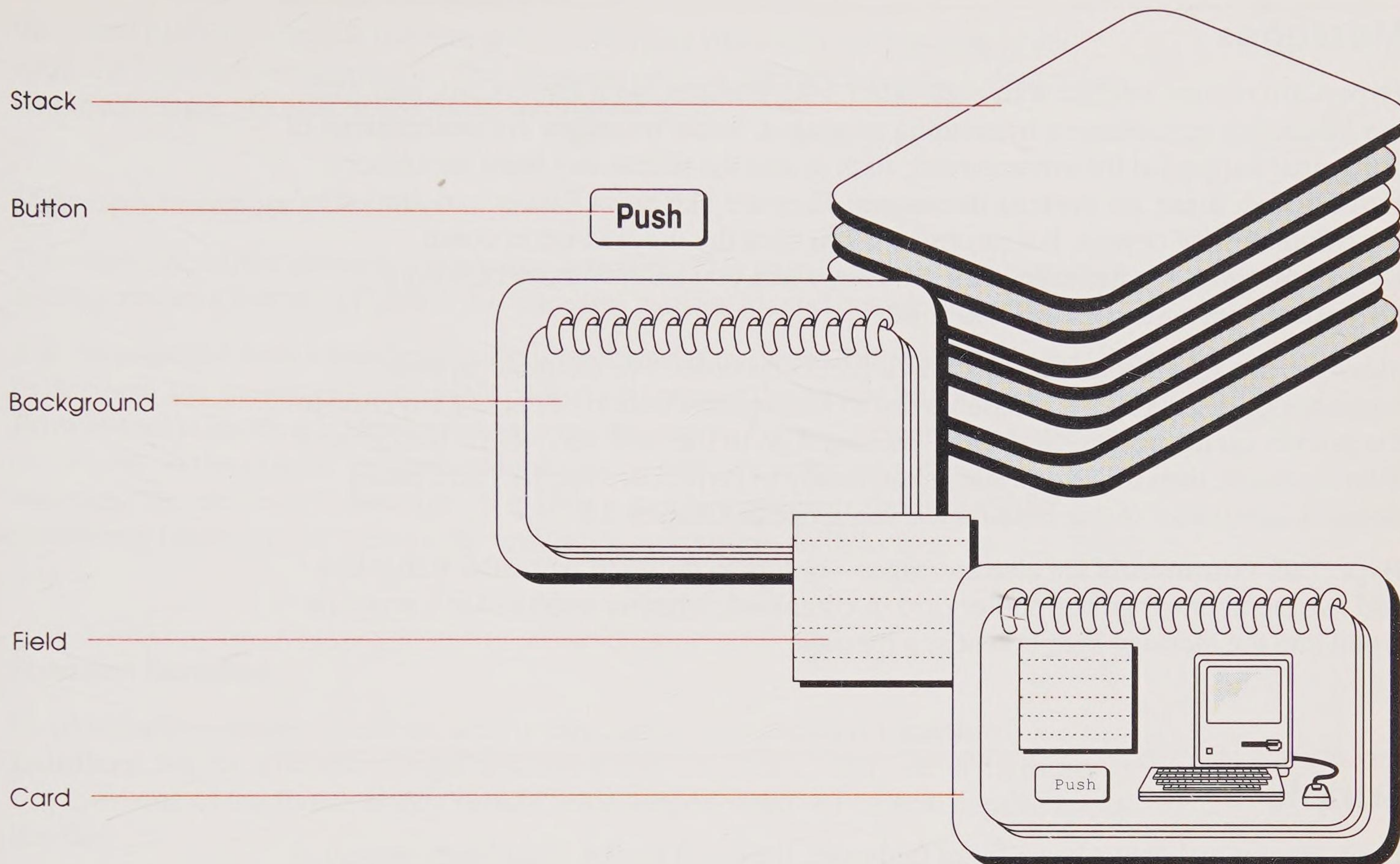
Figure 1-1 HyperCard objects
