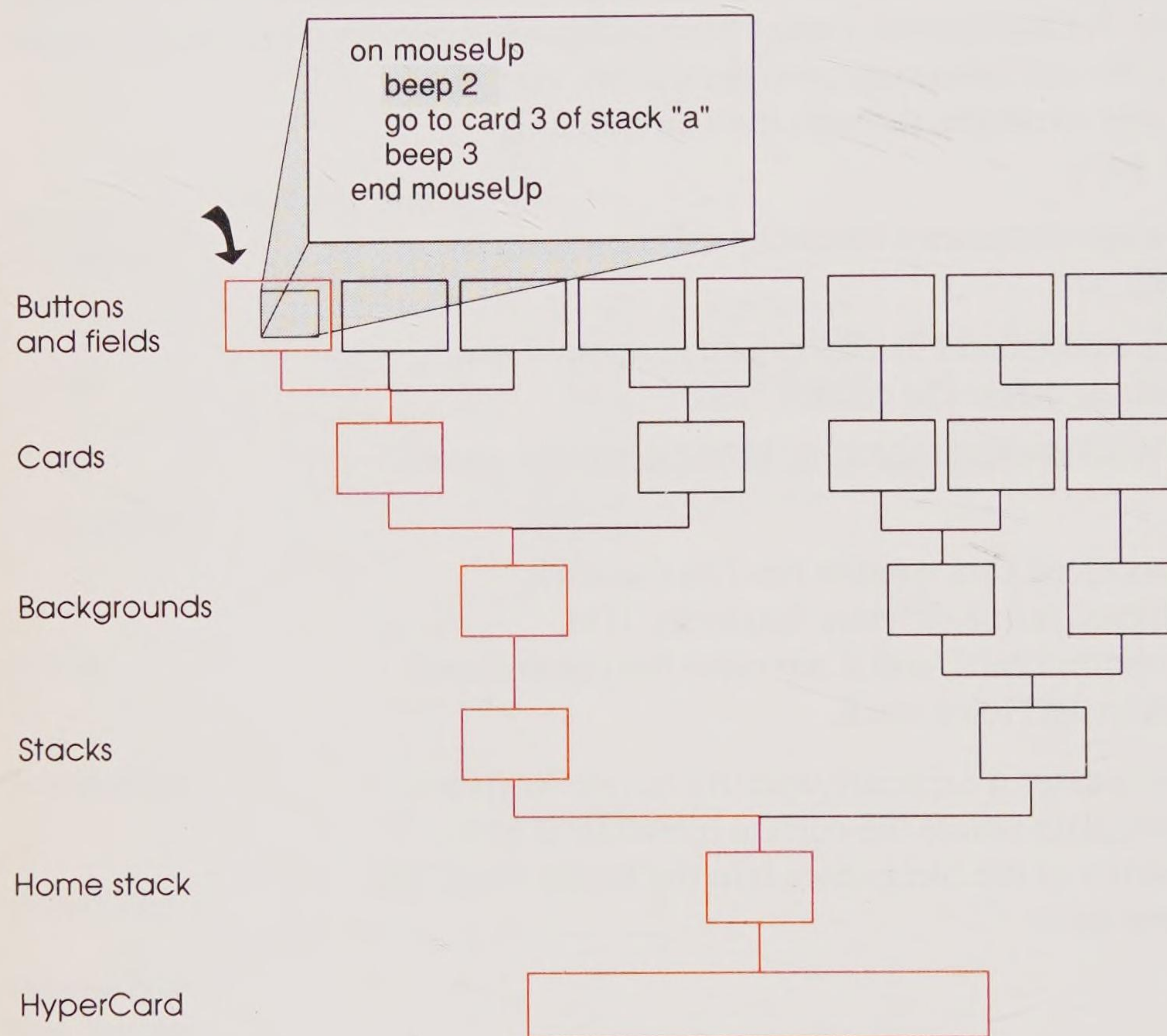
Figure 2-7
