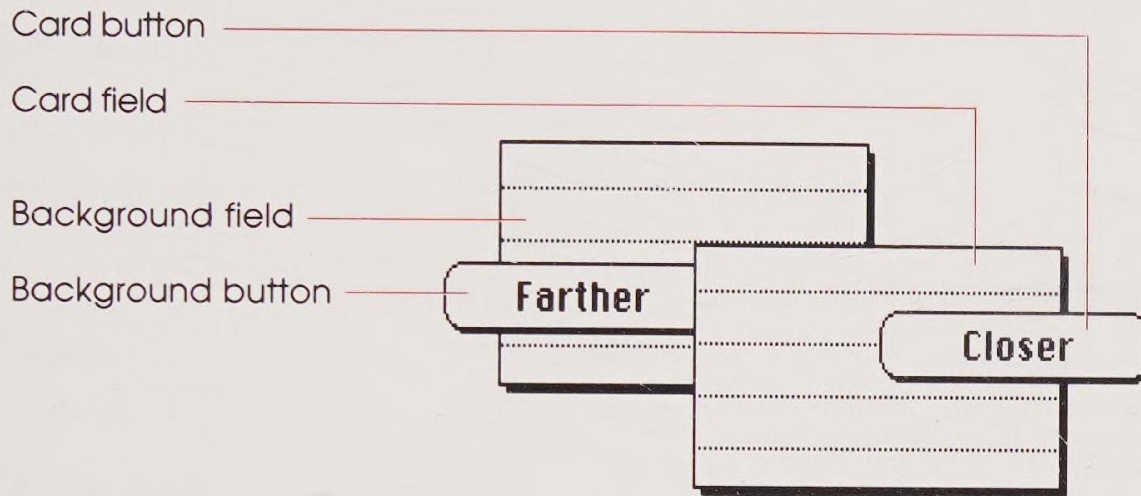
Figure 2-3
