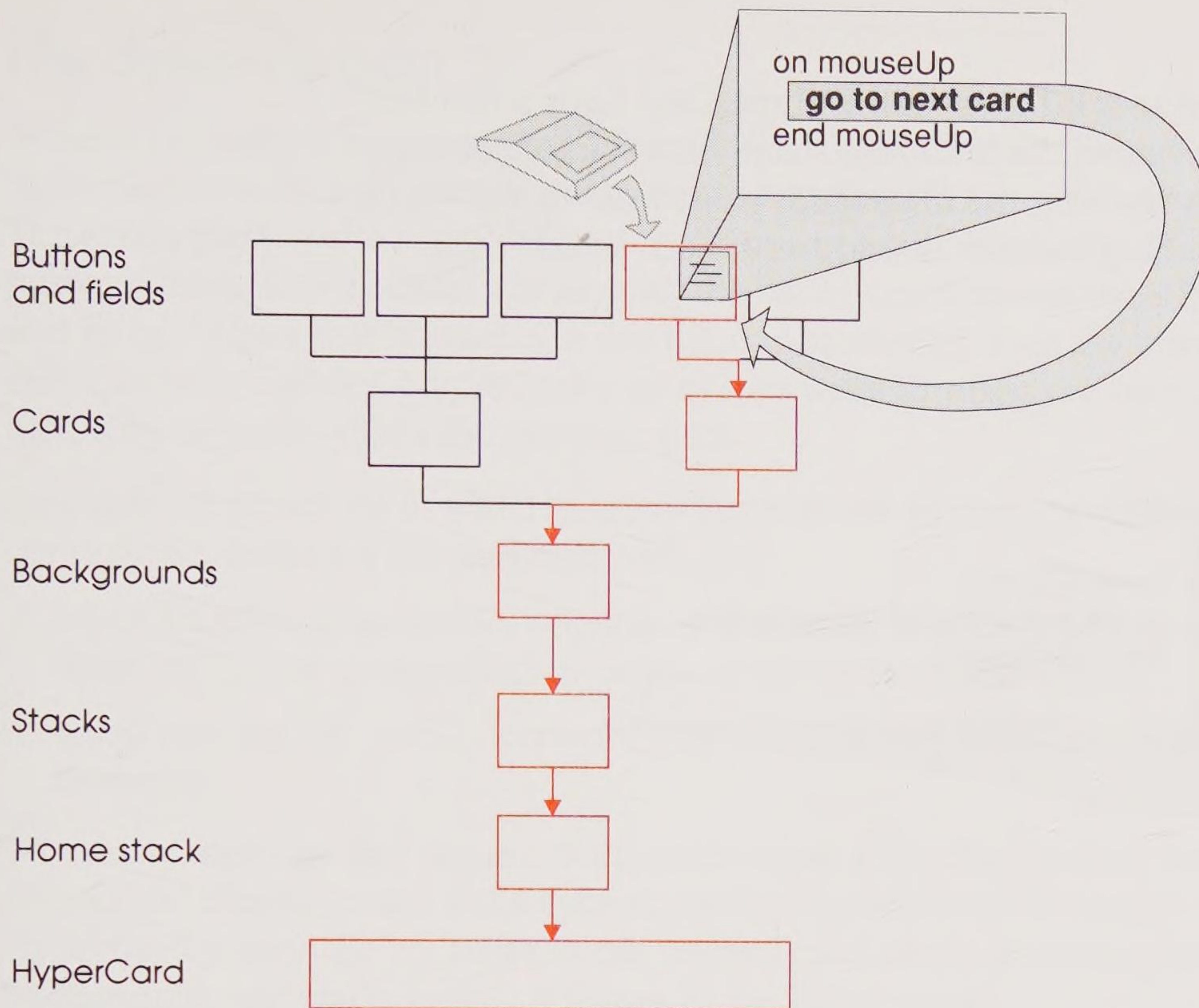
Figure 2-5 Command sent as a message
