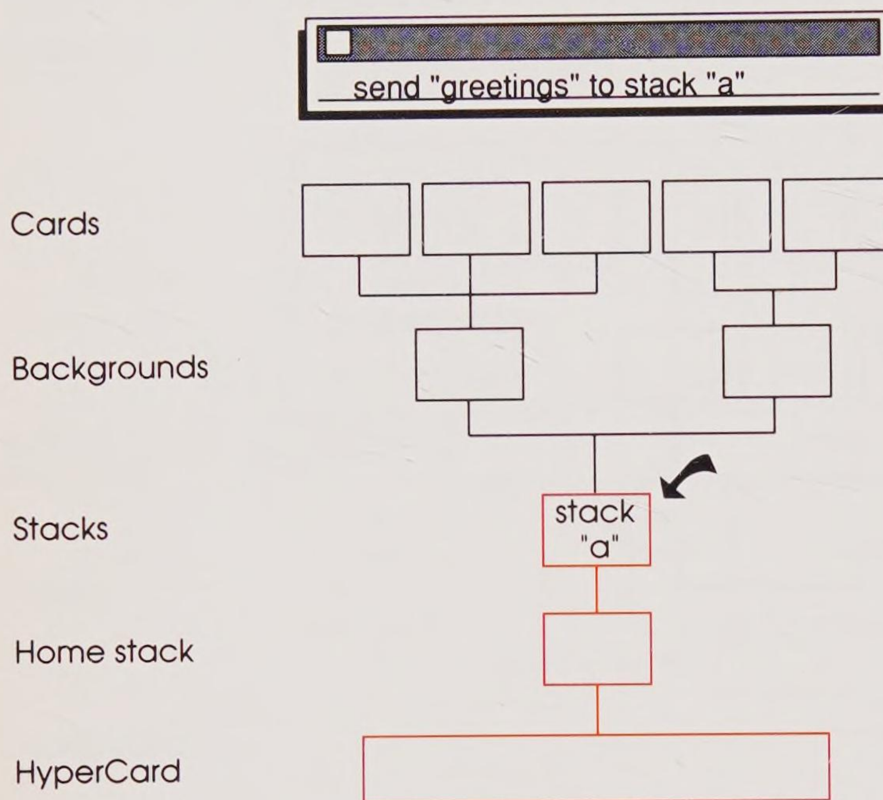
Figure 2-9 Using the send keyword
