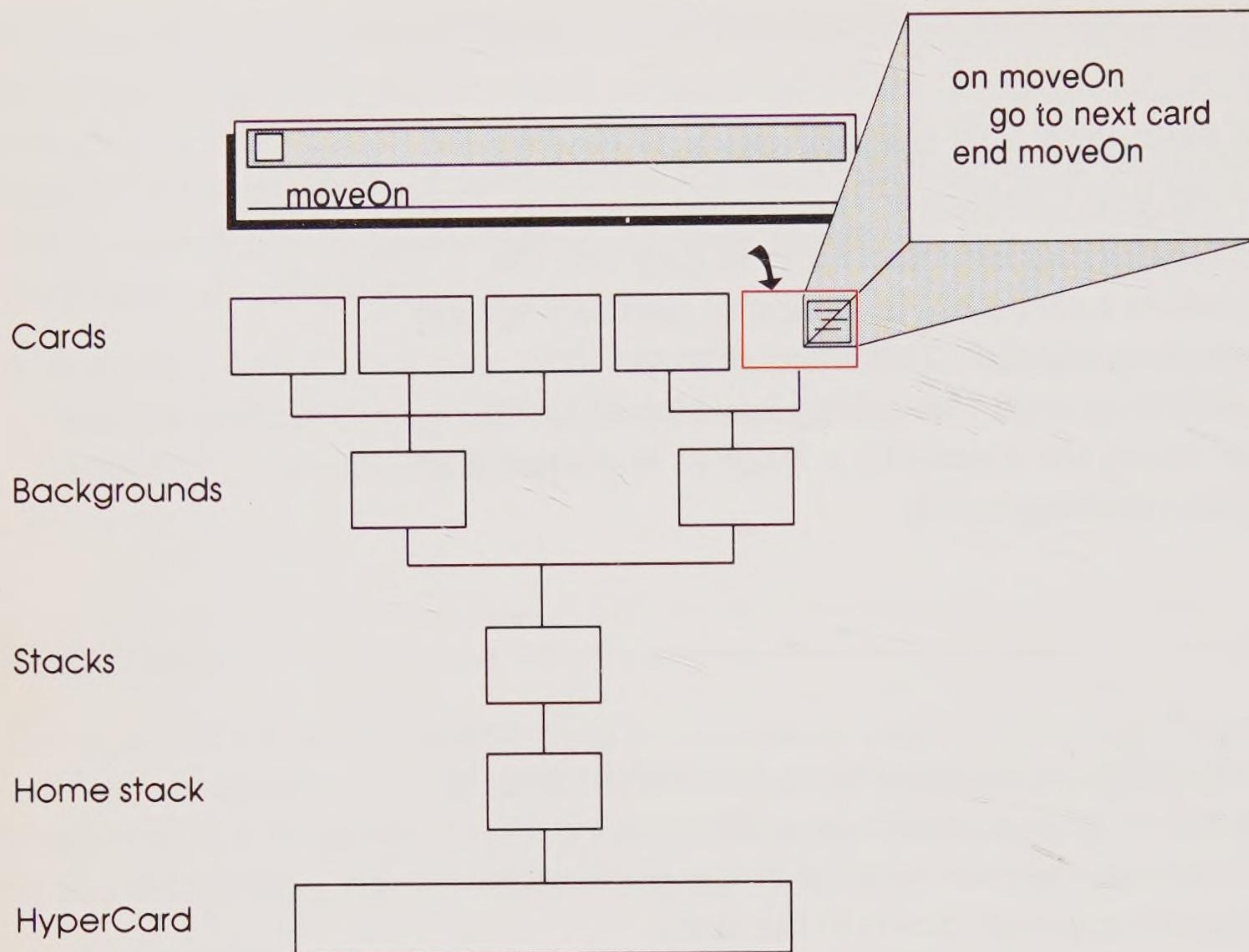
Figure 2-10 Handler in card script
