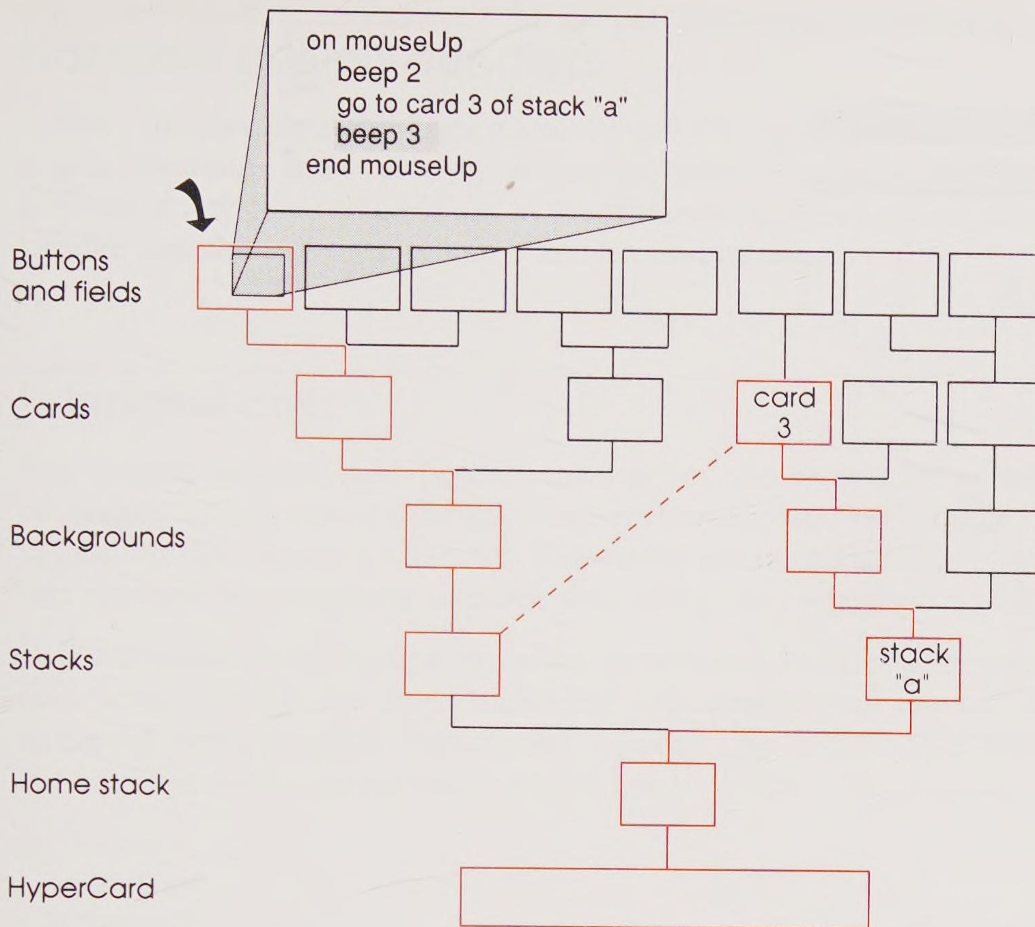
Figure 2-8 Dynamic path after the go command executes
