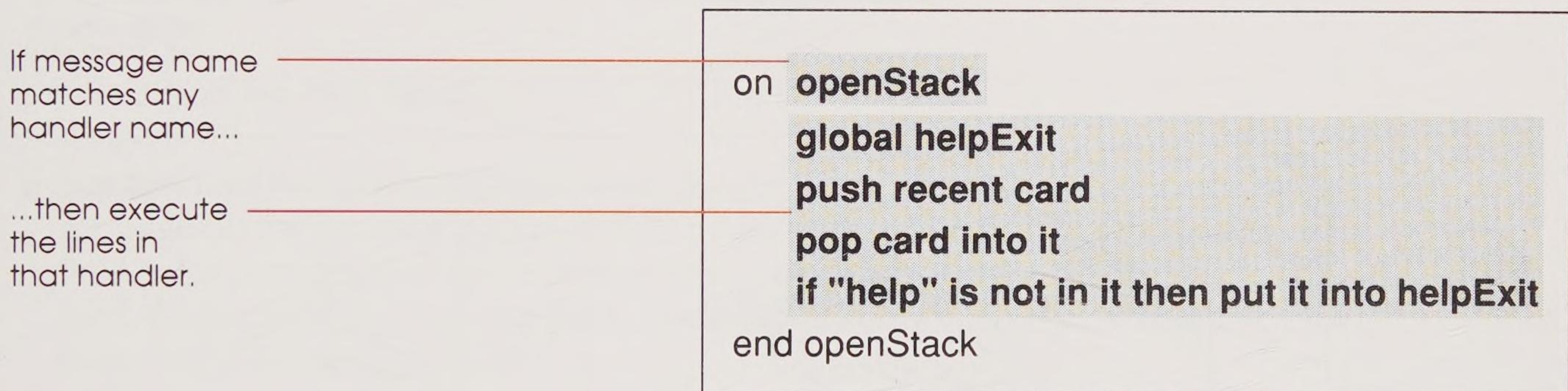
Figure 2-1 Matching messages with handlers
