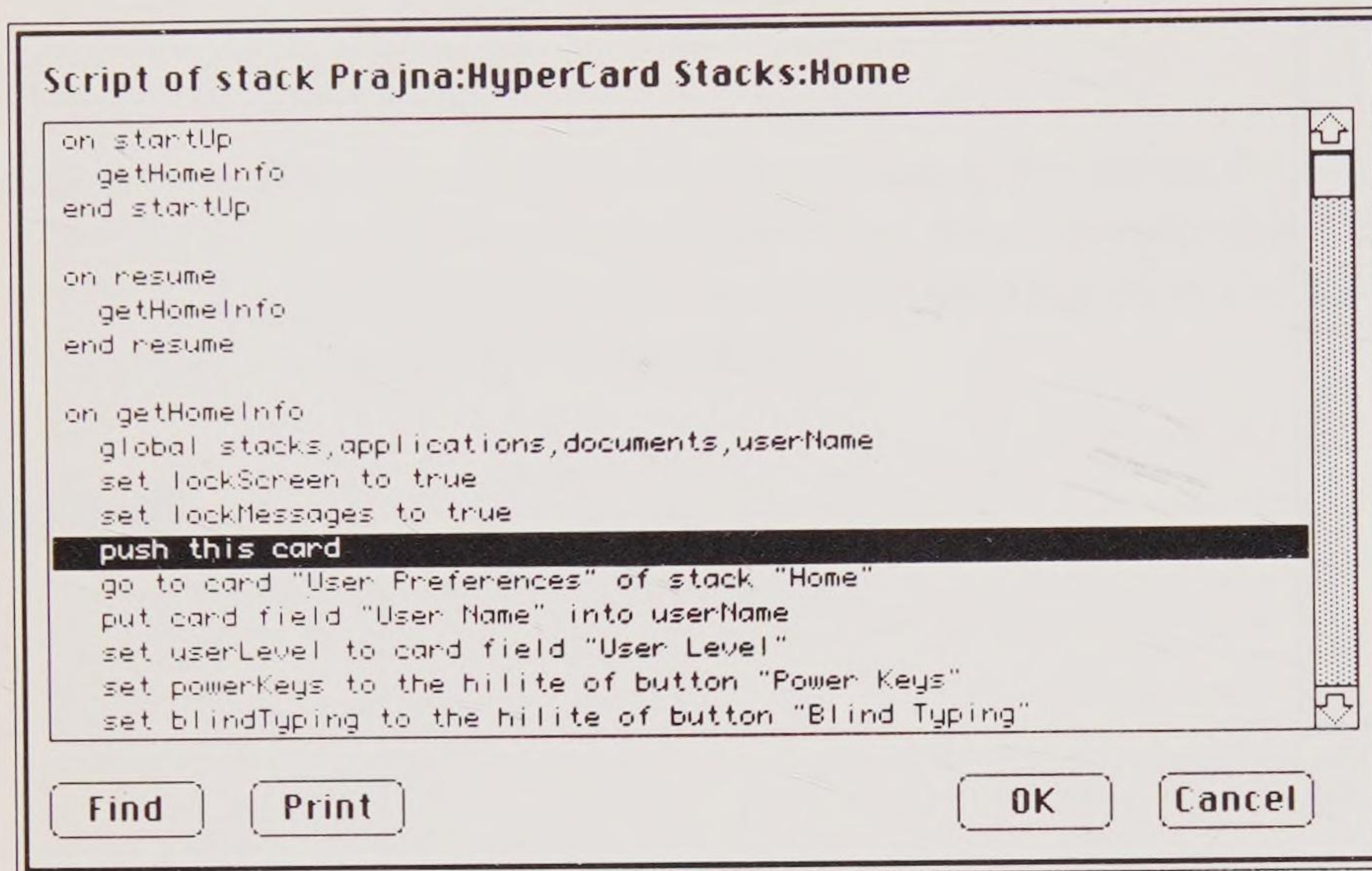
Figure 1-4 Script editor box
