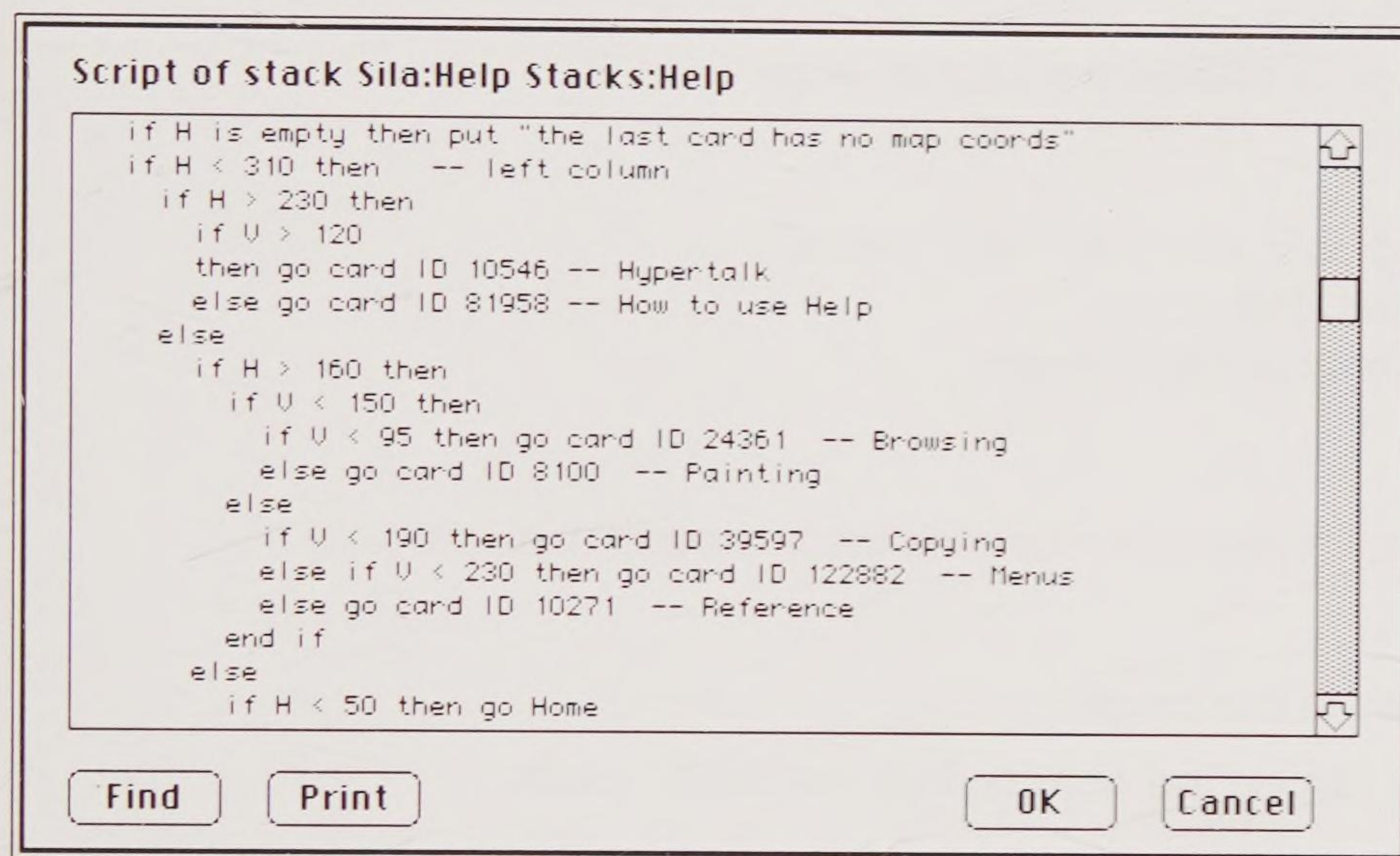
Figure 1-5 Nested control structures
