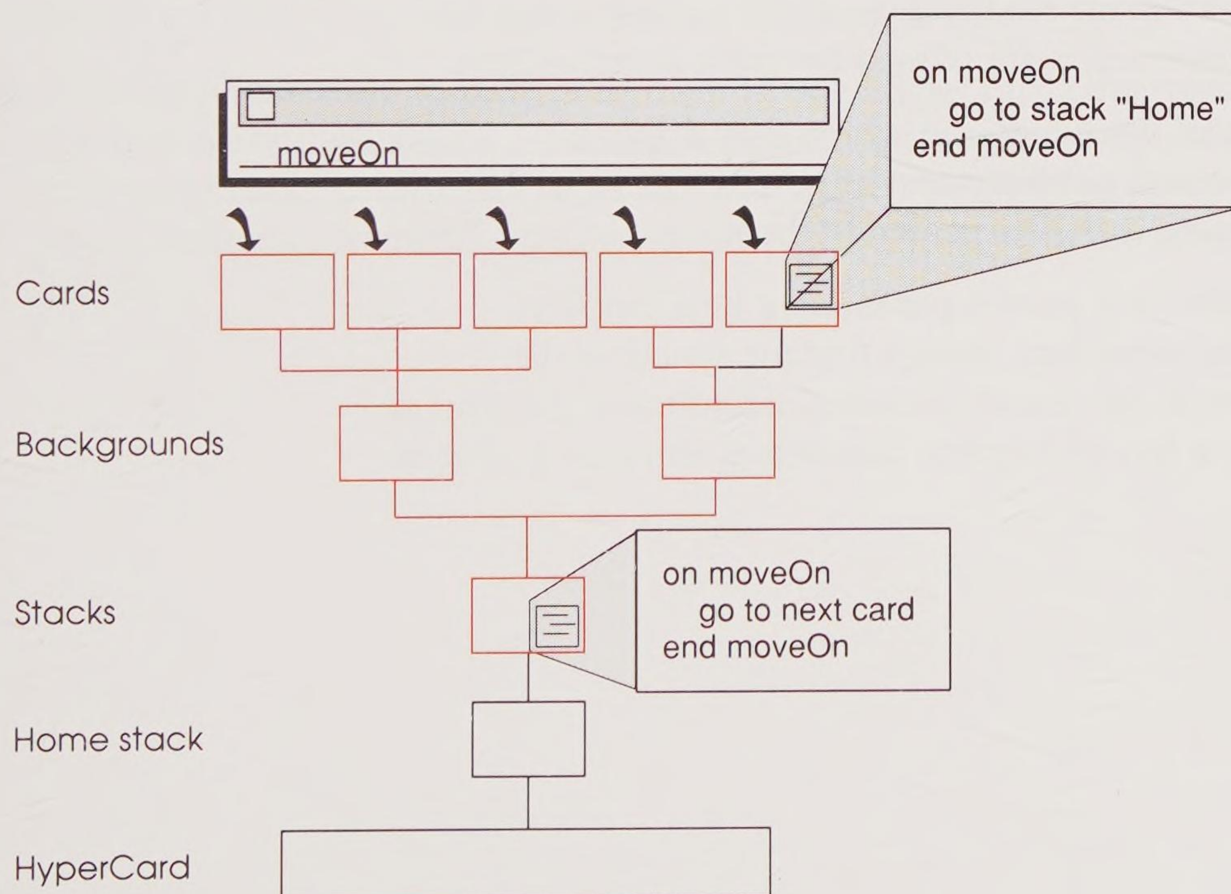
Figure 2-12 Intercepting a message
