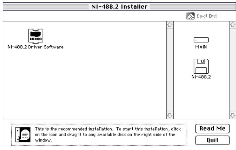
Figure 2-3. Installer Window
